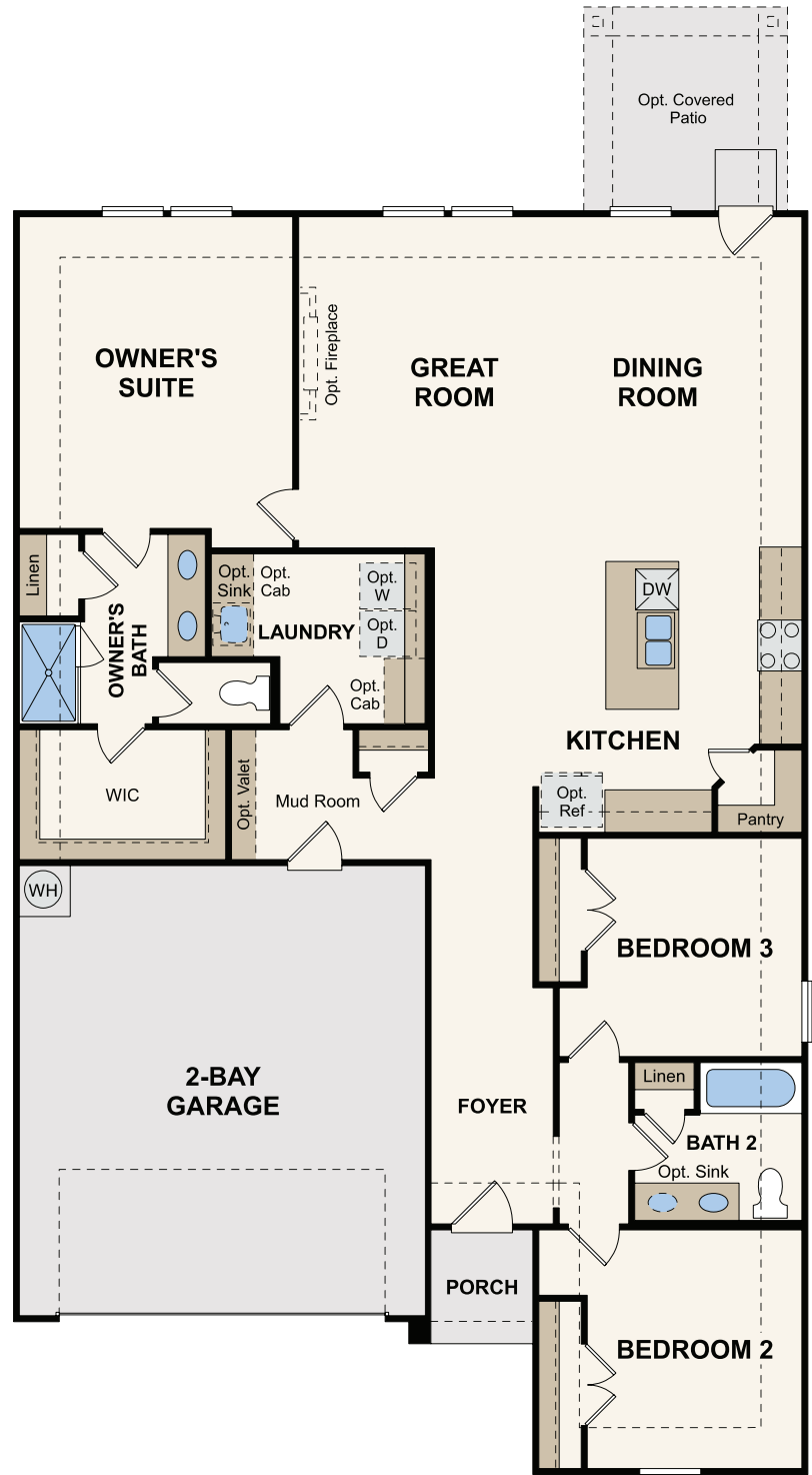
FLOOR PLAN
